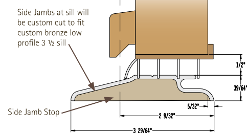
Sill Detail C/W Sweep (2 1/4 also available)
