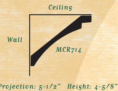
MCR714 Ceiling Step
