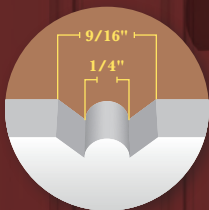
Large Standard Bead (3" On Center), Cap Combination: 1x4, SC214, FS312
