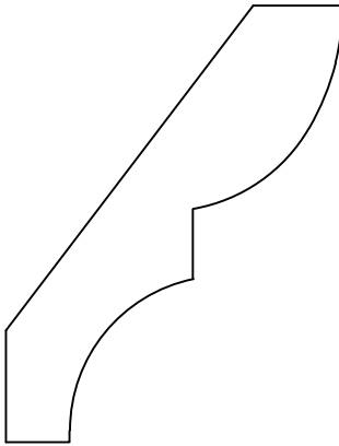
Bed Moulding TL-71 9/16" x 2-5/8" 800.66.TAGUE
