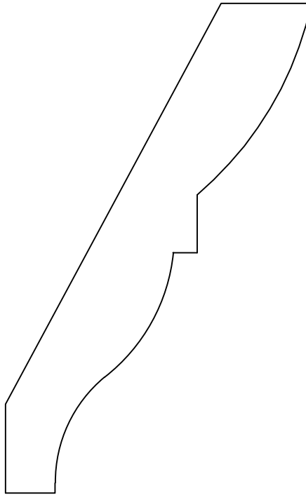
Bed Moulding TL-5 11/16" x 4-1/4" 800.66.TAGUE
